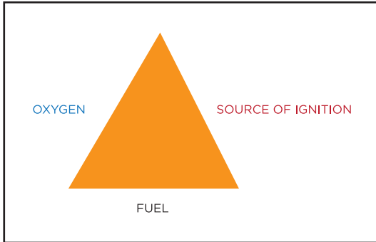
Fire triangle
